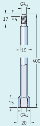
G 1/4 extension pipe
